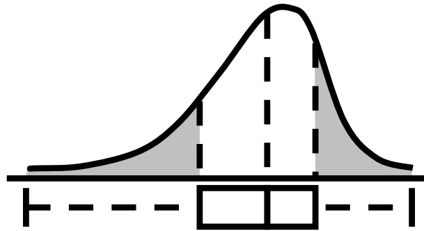
Left-skewed distribution
